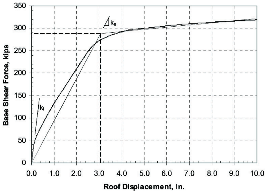
Figure 10 Capacity curve obtained in the pushover analysis of a wall.
