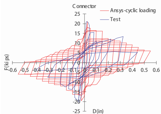
Figure A3-3 Lehigh Phase 1 test specimen and sample results for cyclic shear response (test & FE model) (right).
