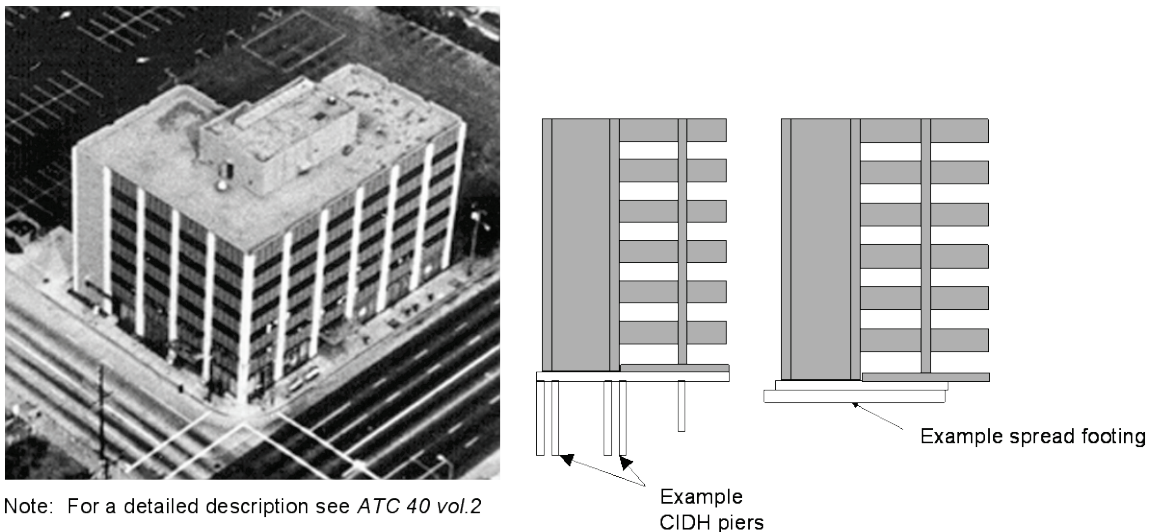
Figure C-A7.2.3-5 Example building.
