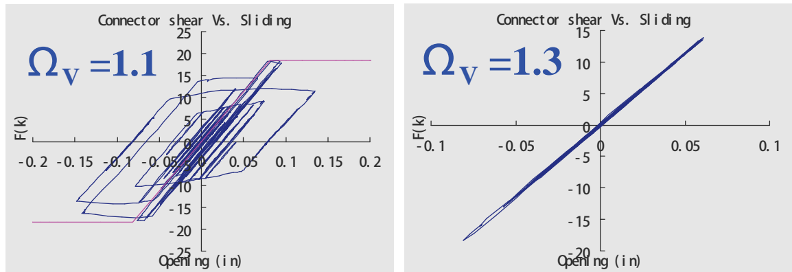
Figure A3-5 Sample results for critical shear connector, \Psi_D = 1.5 Berkeley MCE: (a) \Omega_v = 1.1 , (b) \Omega_v = 1.3 . deformation demand.
