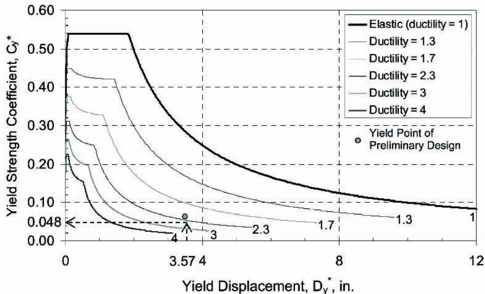
Figure 12 YPS used in the reinforced concrete frame example.
