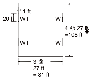
Figure 7 Reinforced concrete wall building plan.
