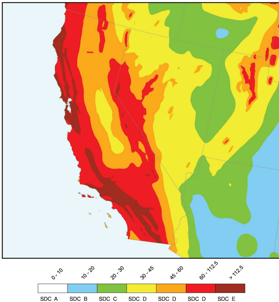
Figure C11.4-3 Map illustrating values of the MCE R 1-second spectral response acceleration parameter, S M1 (%g), and associated regions of Seismic Design Category, assuming Site Class D conditions, for California sites.
