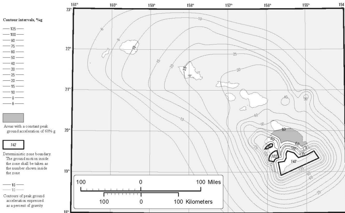
Figure 22-10 MCE geometric mean PGA, %g, Site Class B for Hawaii
