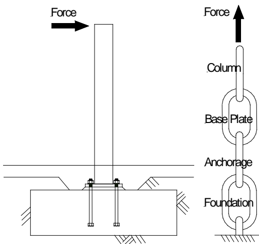
Figure 1 Structural elements in series (column, base plate, anchorage, foundation, and soil).
