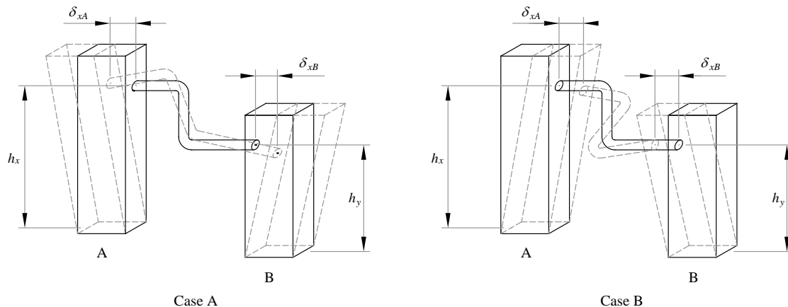
Figure C13.3-4 Displacements between structures.
