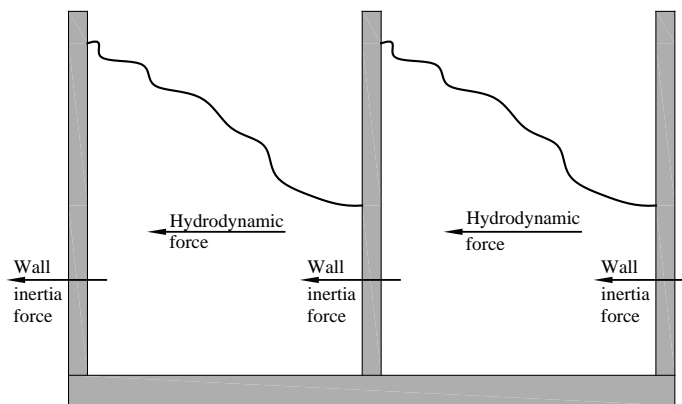
Figure C15.6-1 Wall forces.
