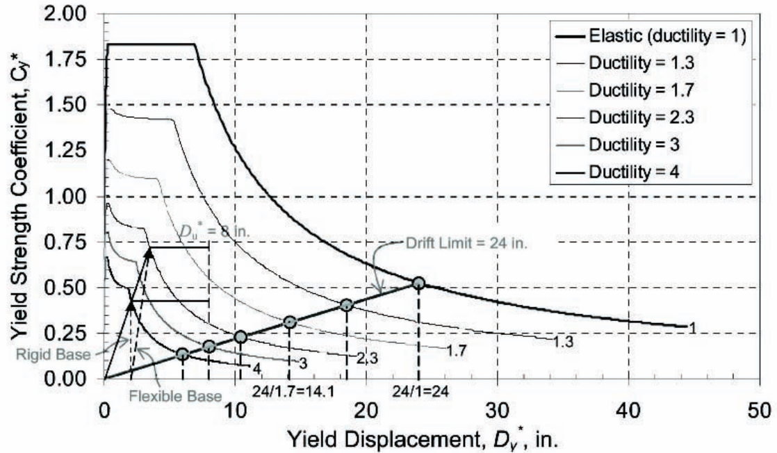
Figure 16 Establishment of the drift limit and illustration of the influence of foundation flexibility on response and required strength.
