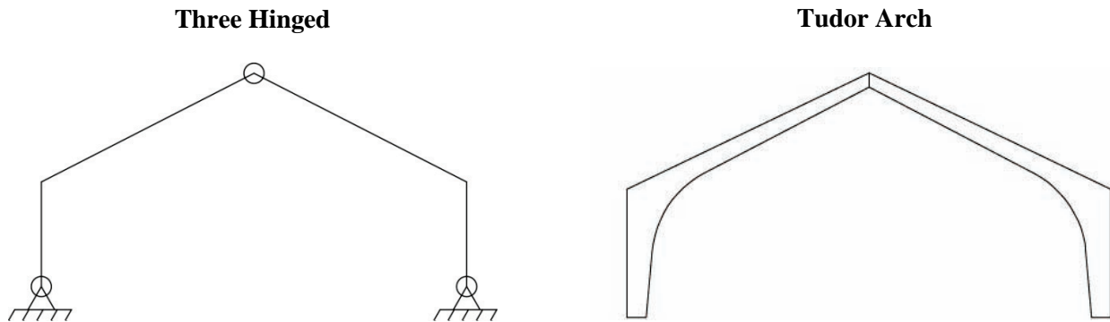
Figure C1.0 Three-hinge arch and Tudor arch configurations.
