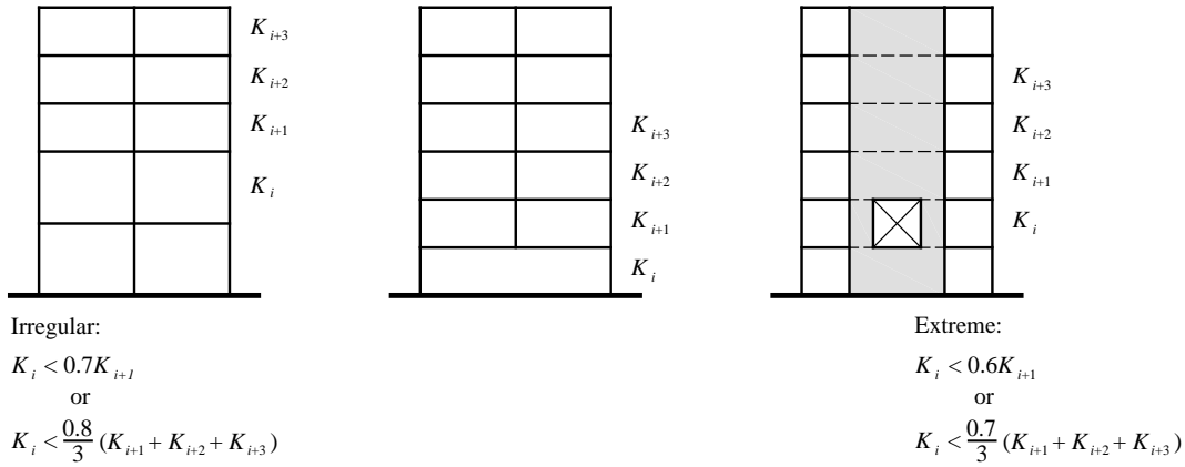
1. Stiffness – Soft Story
