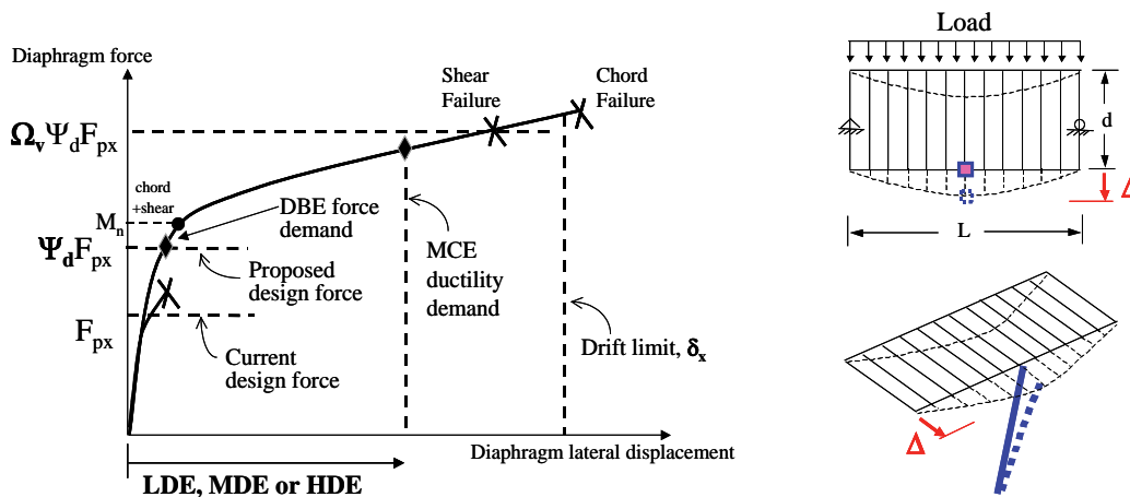
Figure 1 Diaphragm response curve (left) and diaphragm force and deformation (right).
