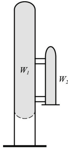
Figure C15.1-7 Torsional irregularity.
