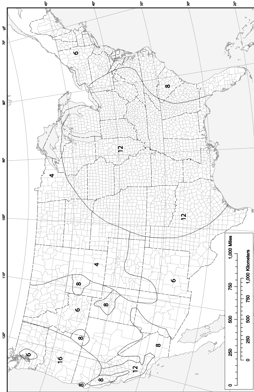
Figure 22-7 Long-period transition period, T_L (s)
