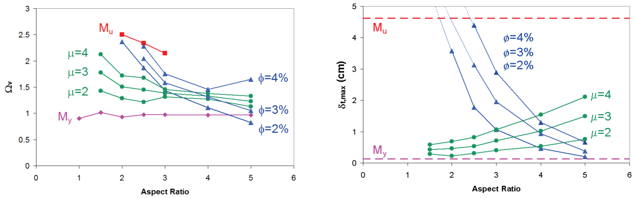
Figure A3-2 Design charts: \Omega_v vs. aspect ratio (left) and deformation capacity c vs. aspect ratio (right).
