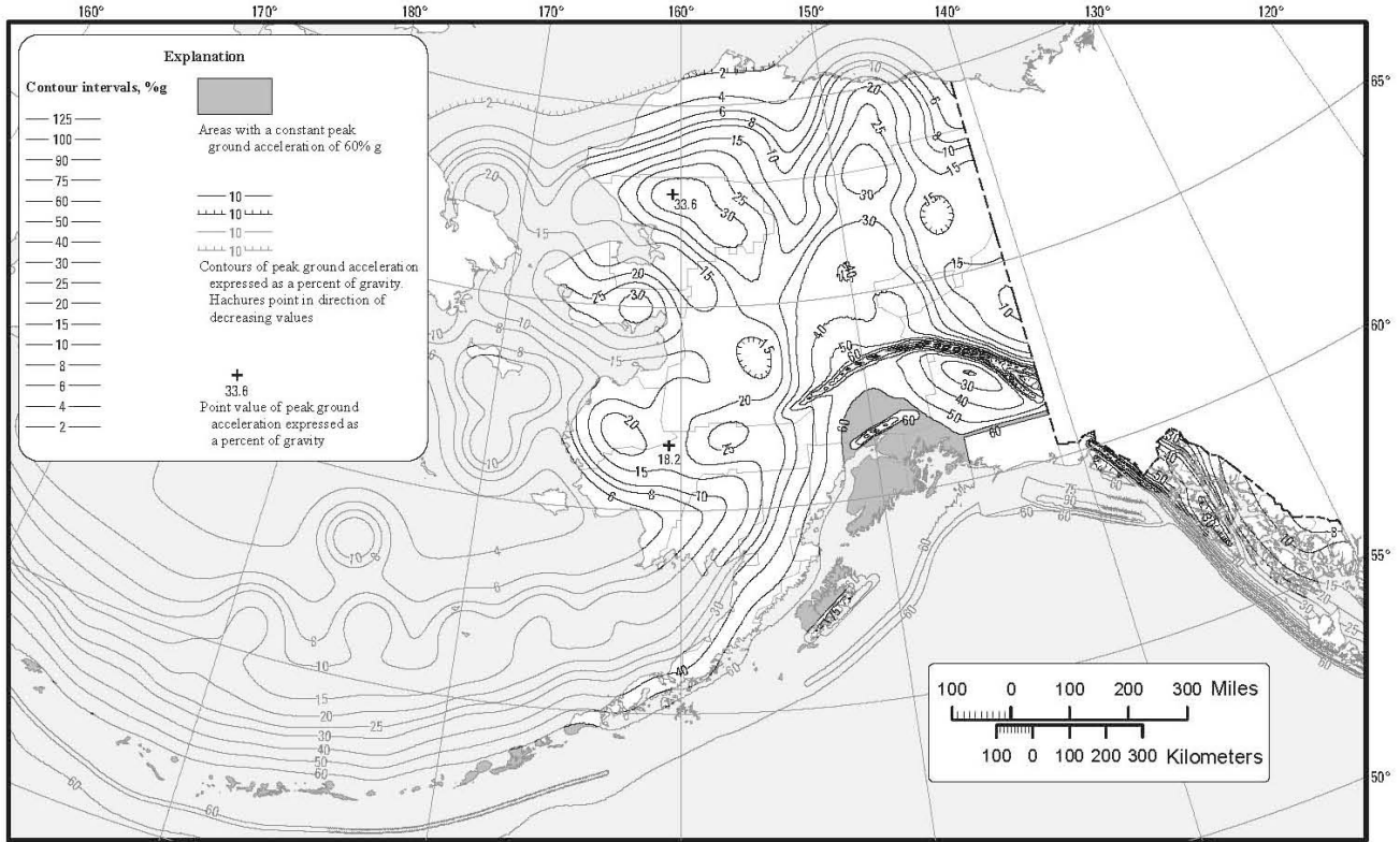
Figure 22-9 MCE geometric mean PGA, %g, Site Class B for Alaska
