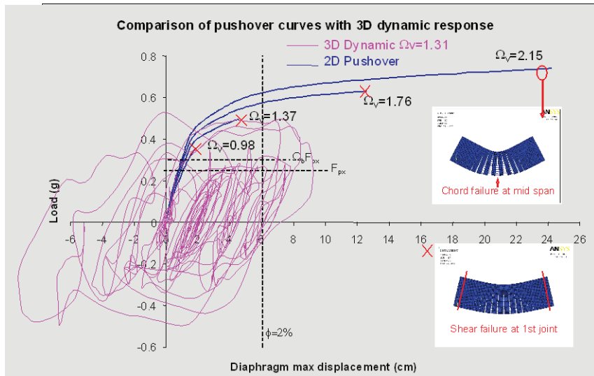
Figure A3-4 Superposition of 3D-FE global EQ demand results on 2D pushover.
