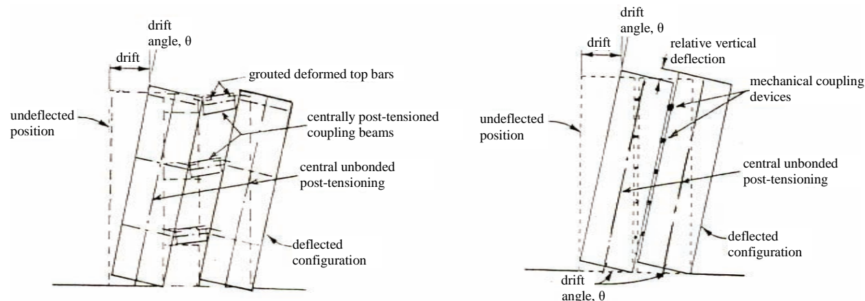
Figure C14.2.4.5.1 (a) Coupled wall test module with coupling beams; (b) Coupled wall test module with vertical mechanical couplers.
