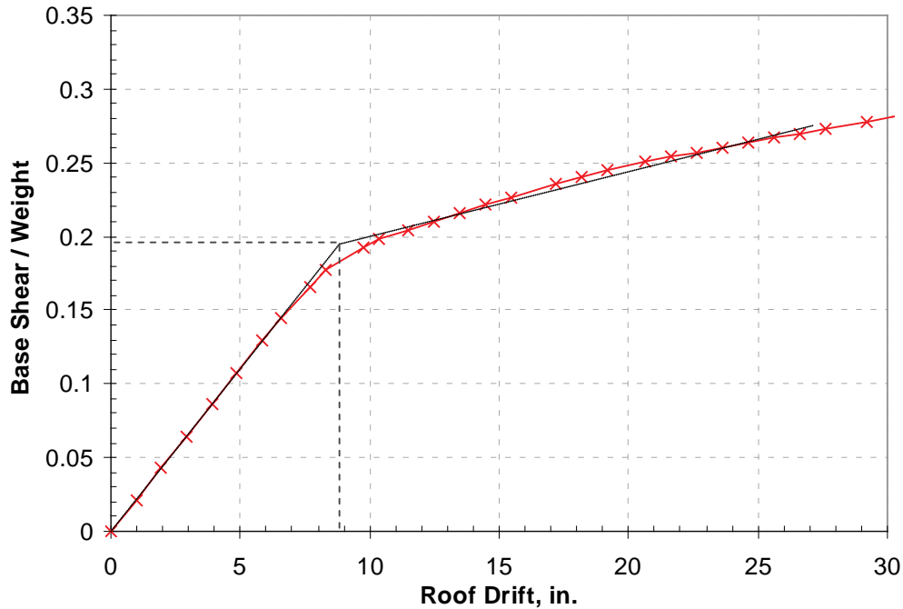
Figure 4 Capacity curve obtained from a nonlinear static (pushover) analysis.
