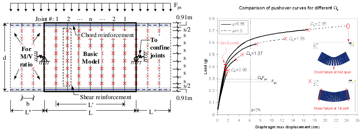
Figure A3-1 Schematic of 2D FE model (left) and sample results for diaphragm shear overstrength factor \Omega_v .
