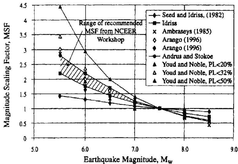
Figure 5 Magnitude scaling factors derived by various investigators (NCEER, 1997; Youd et al., 2001).
