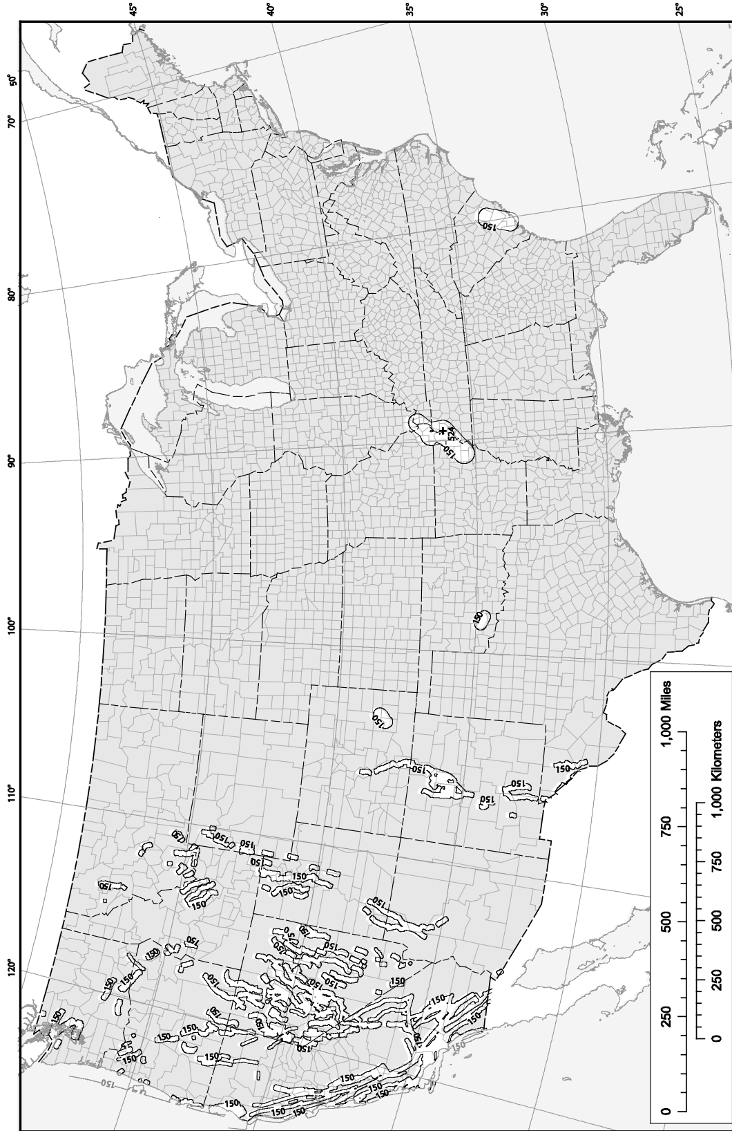
Figure 22-5 Deterministic ground motions of 0.2-second spectral response acceleration (5% of Critical Damping), Site Class B
