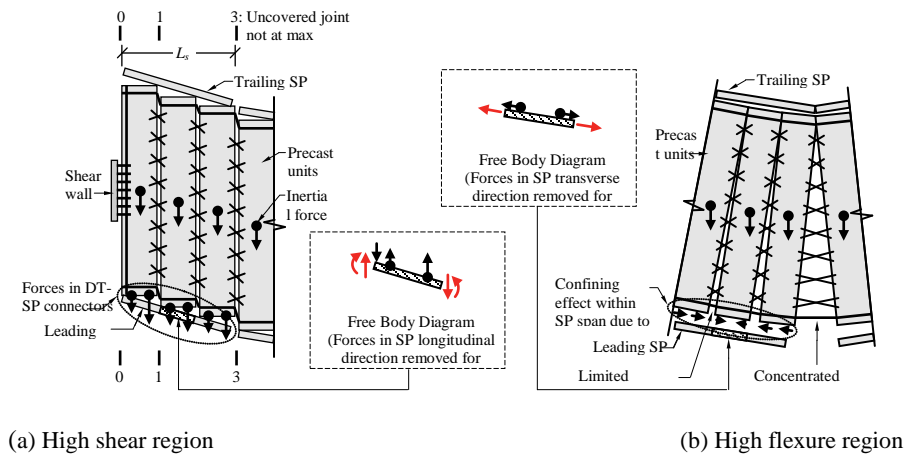
Figure A6-1 Schematics of interaction between spandrels and precast floor units.
