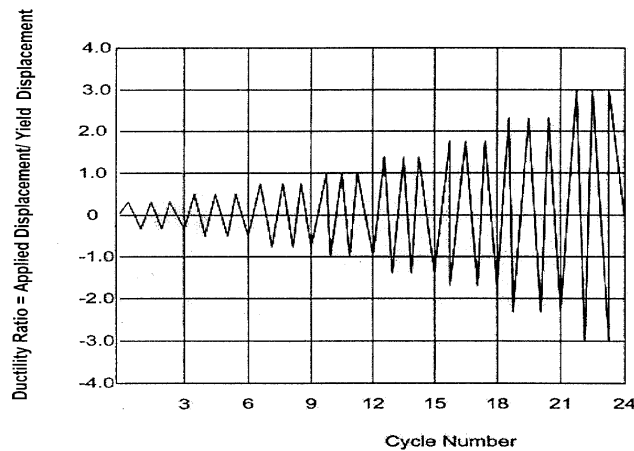
Figure A4-3 Example of specified test sequence.
