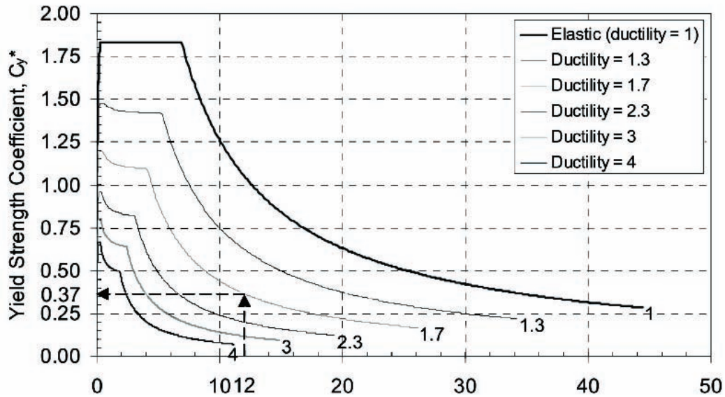
Figure 6 Yield point spectra.
