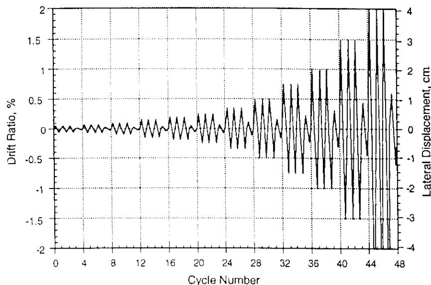
Figure C14.2.4.7 Example of specified test sequence.
