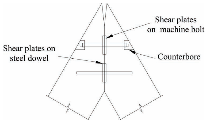
Figure C1.1.2 Typical arch peak connection detail.
