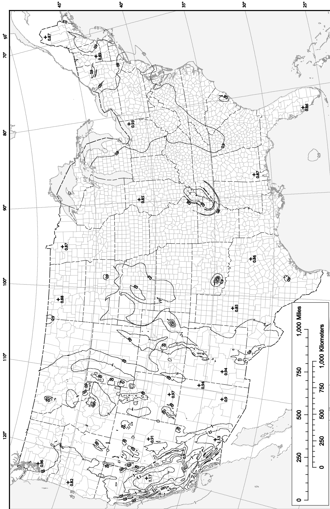
Figure 22-4 Risk coefficient at 1.0-second spectral response period
