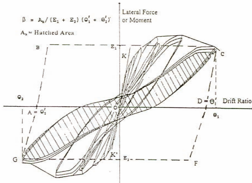
Figure C14.2.4.2.5 Relative energy dissipation ratio.
