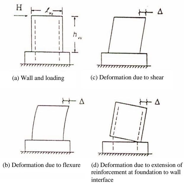
Figure C14.2.4.2.2-2 Typical wall deformation components.
