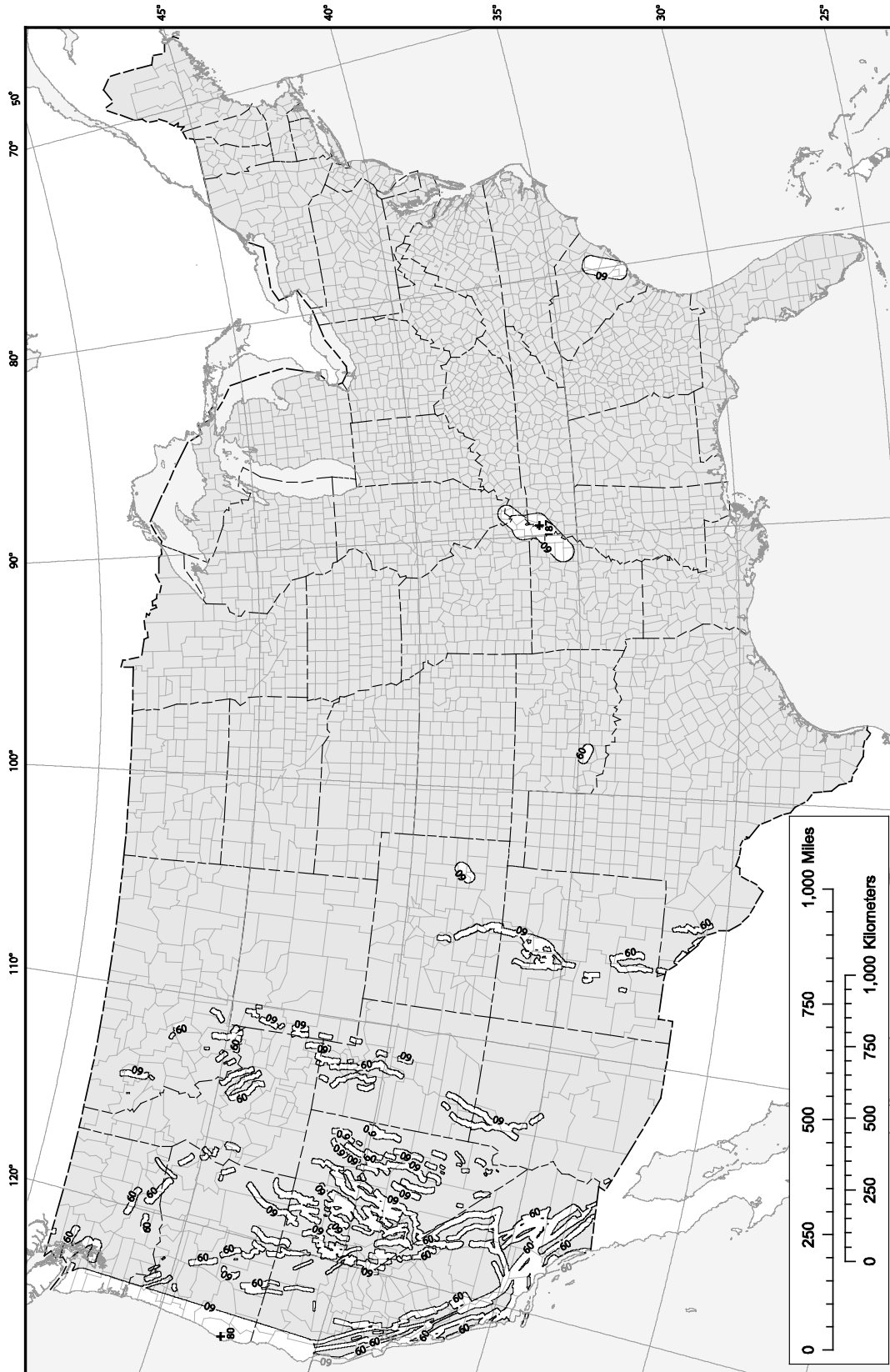
Figure 22-6 Deterministic ground motions of 1.0-second spectral response acceleration (5% of Critical Damping), Site Class B
