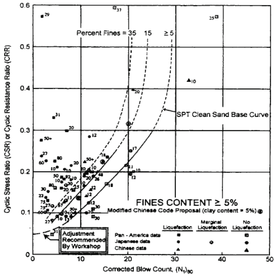
Figure 4 SPT clean sand base curve for magnitude 7.5 earthquakes with data from liquefaction case histories (modified from Seed et al., 1985, to reflect NCEER, 1997, and Youd et al., 2001).
