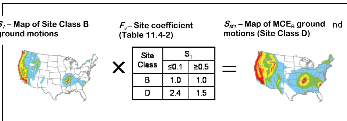
Figure C11.4-1 Illustration of process for developing 1-second MCE_R Site Class D ground motions using formulas of Section 11.4.3 and associated mapped values of ground motions and risk coefficients of Chapter 22.
