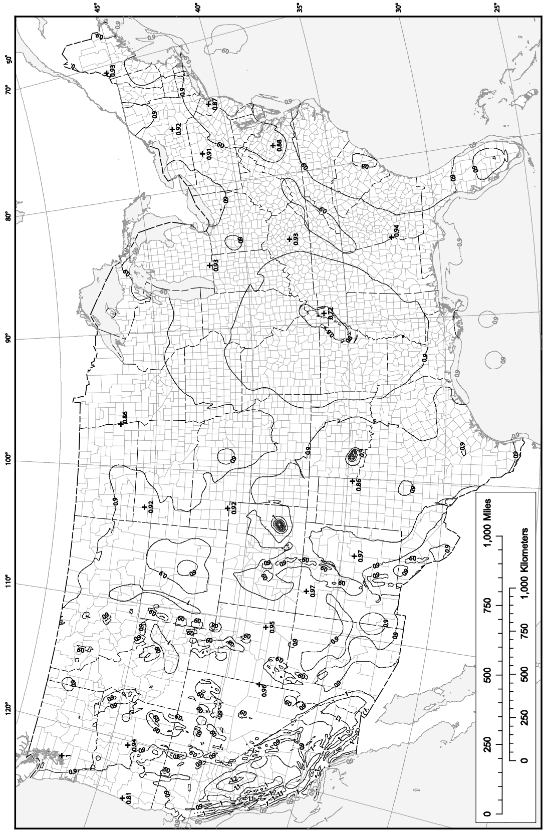
Figure 22-3 Risk coefficient at 0.2-second spectral response period
