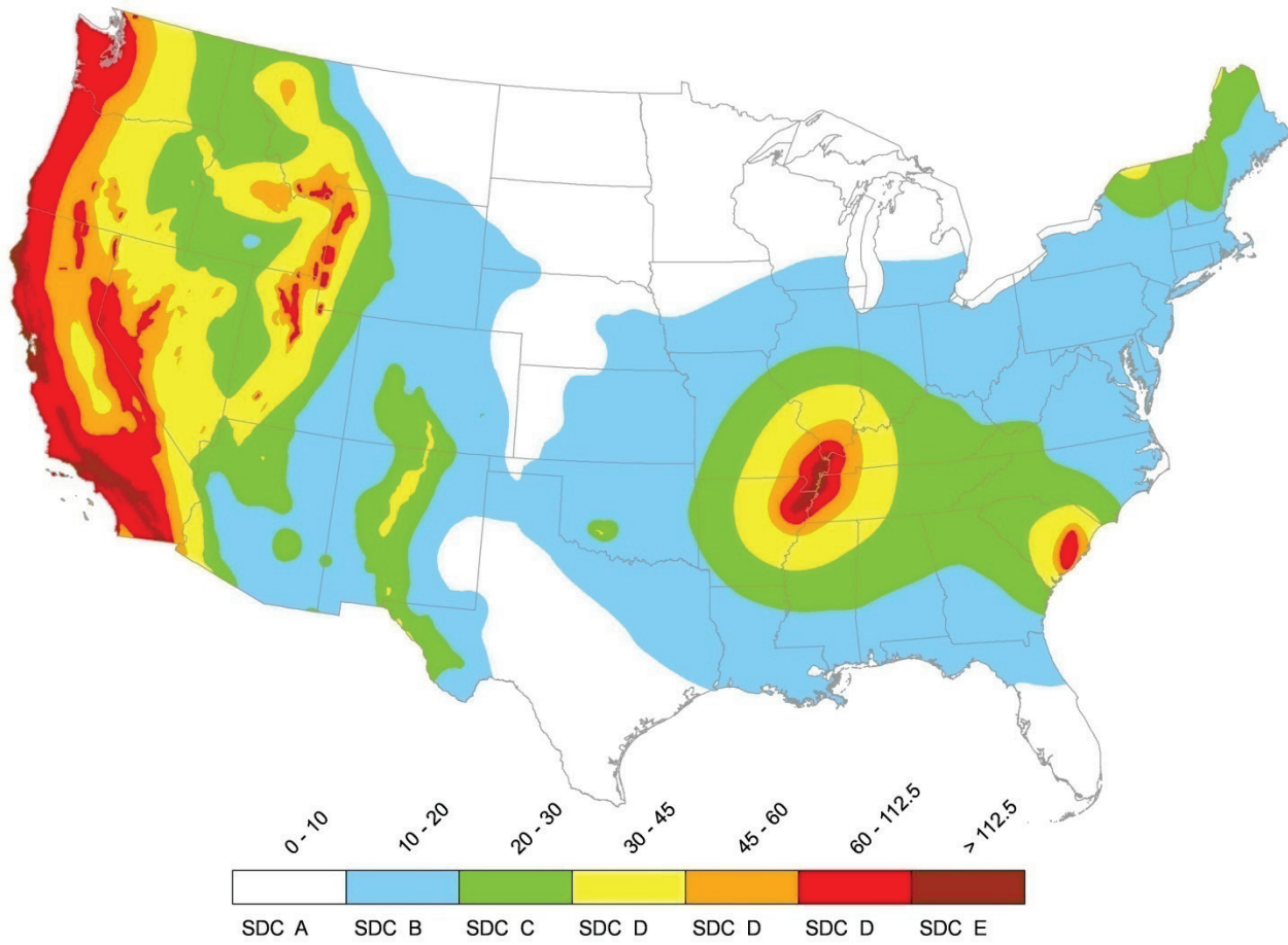
Figure C11.4-2 Map illustrating values of the MCE R 1-second spectral response acceleration parameter, S M1 (%g), and associated regions of Seismic Design Category, assuming Site Class D conditions.
