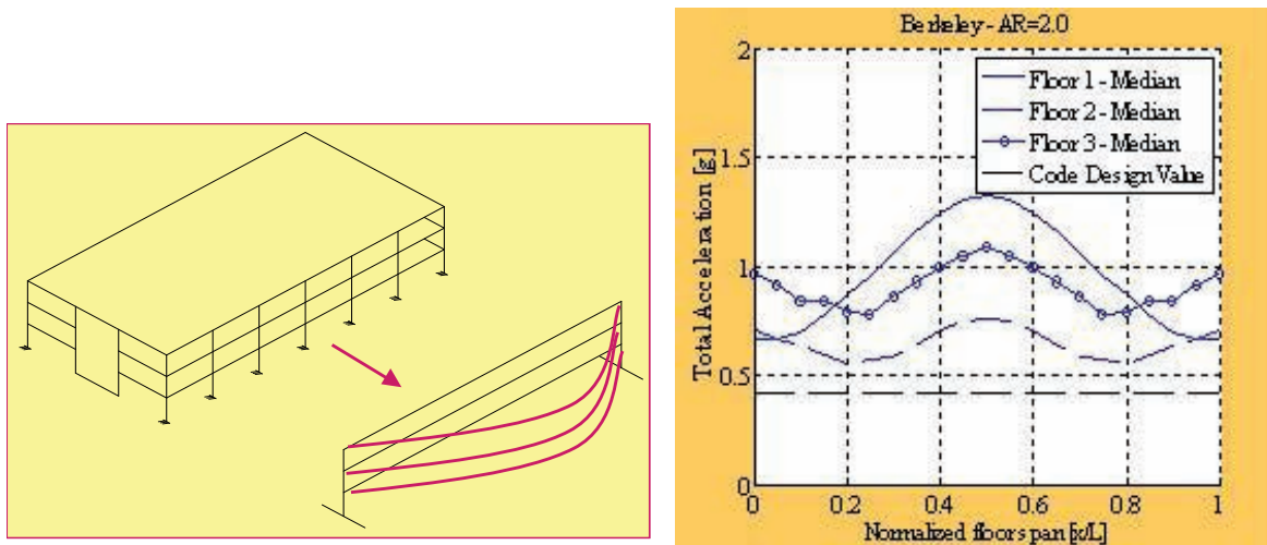
Figure A2-1 Schematic of RDOF model (left) and sample results for the floor (right).
