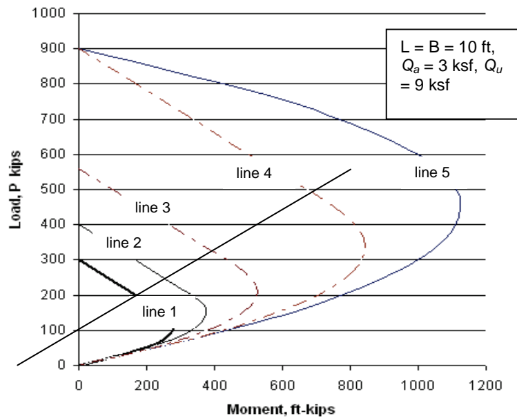
Figure 6 Example interaction curve for a shallow foundation.
