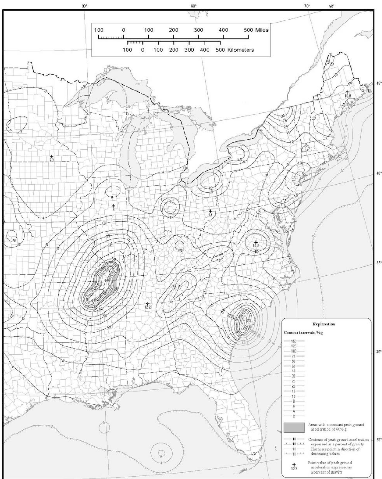
Figure 22-8 (continued) MCE geometric mean PGA, %g, Site Class B for the conterminous United States
