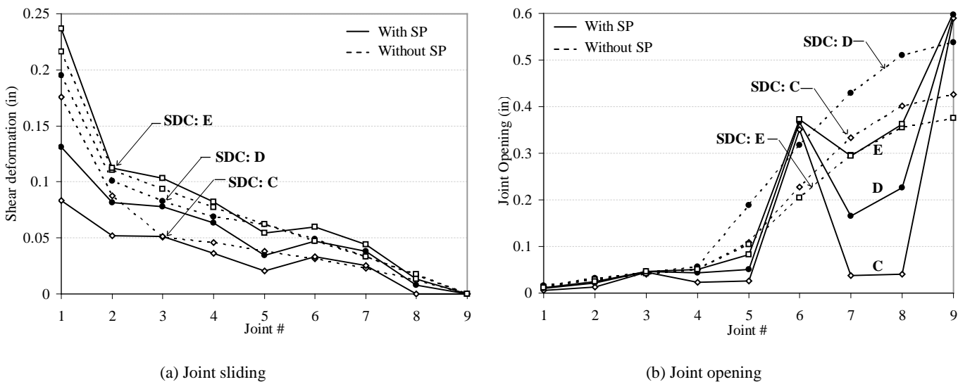
Figure A6-2 Joint deformation profiles including spandrel effects.
