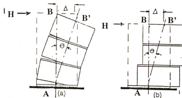
Figure C14.2.4.2.2-3 Undesirable deformations along horizontal joints: (a) excessive gap opening between panels and (b) shear slip.
