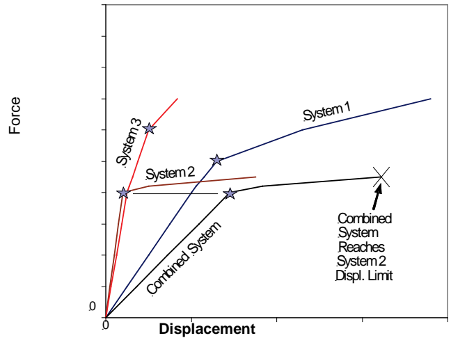
Figure 2 Force versus displacement of series-connected elements.
