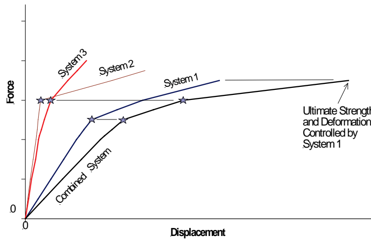
Figure 3 Using load factors to increase required strength of System 2 causes behavior to be controlled by System 1.
