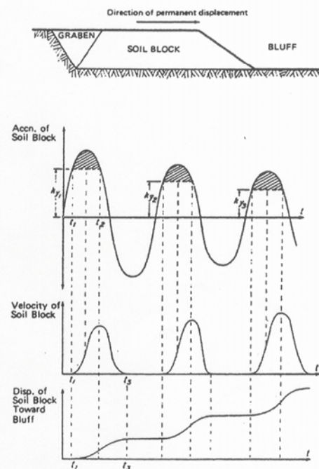
Figure 2 Schematic illustration for calculating displacements of soil block toward the bluff (National Research Council, 1985; from Idriss, 1985, adapted from Goodman and Seed, 1966).
