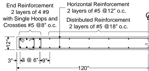
Figure 9 Section at the base of the reinforced concrete wall.
