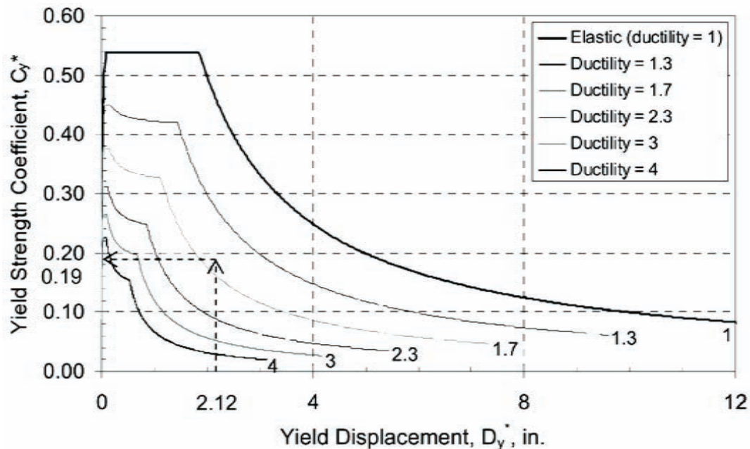
Figure 8 YPS used in the wall building example.
