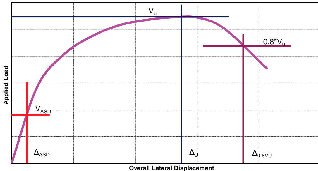
Figure 1-1 Vertical shear wall element parameters.
