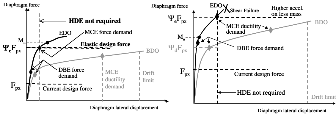
Figure 2 Elastic design option (EDO): low seismic hazard (left) and squat diaphragm geometry (right).
