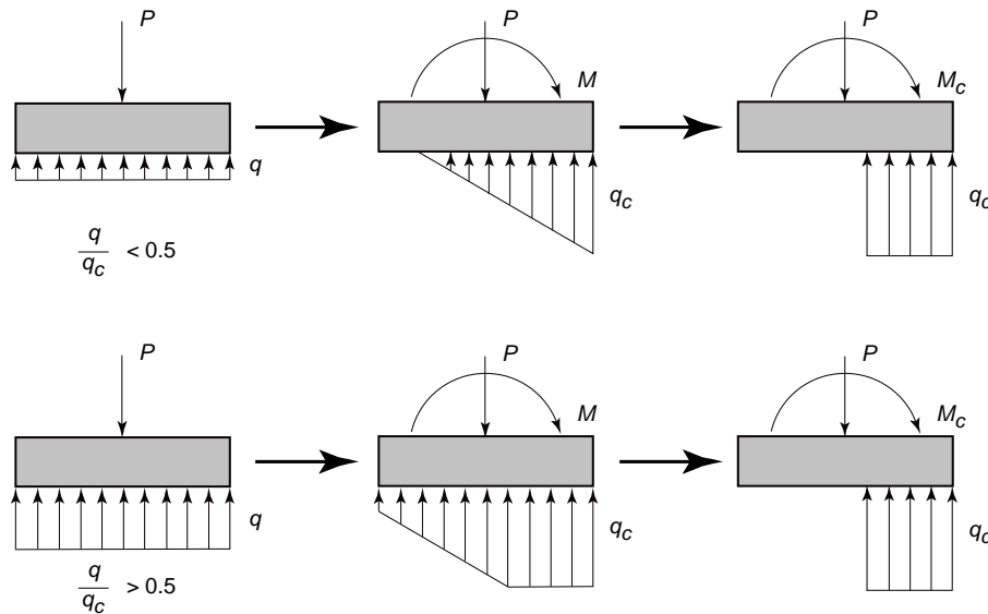
Figure C-A7.2.2-1.
