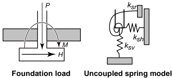
Figure C-A7.2.3-3.
