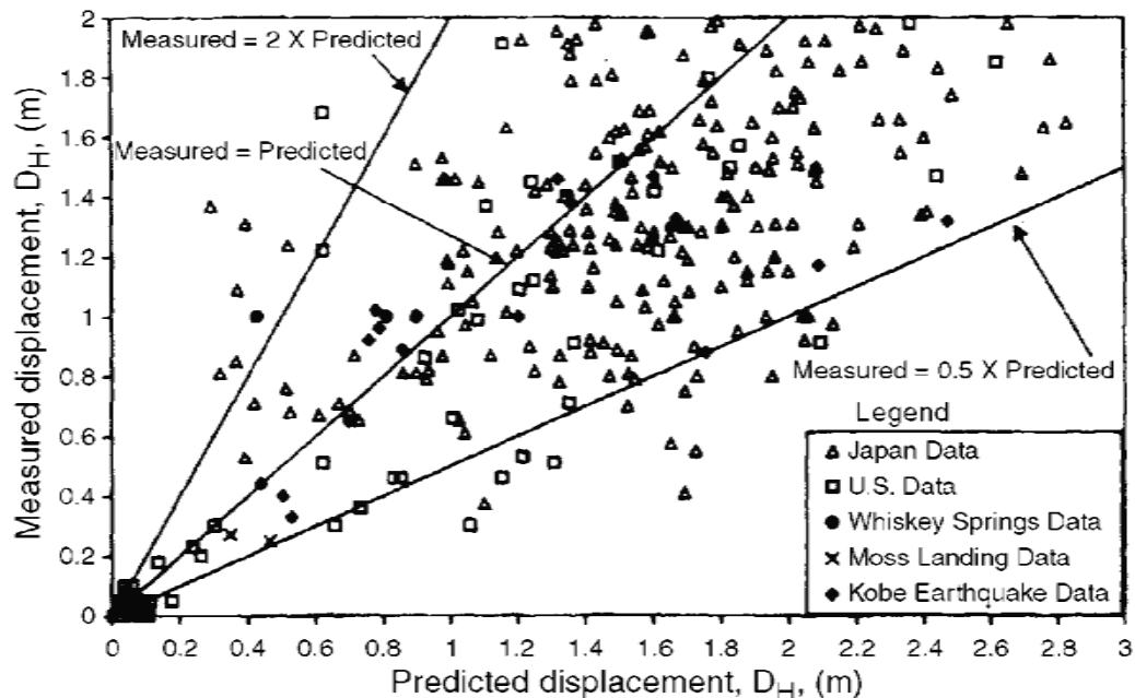
Figure 6 Measured versus predicted displacements for displacements up to 2 meters (Youd et al., 2002).
