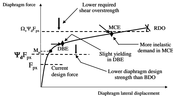
Figure 3 Relaxed design option (RDO).
