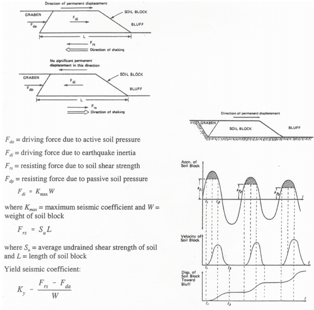
Figure 2 Schematic illustration for calculating displacements of soil block toward the bluff (National Research Council, 1985; from Idriss, 1985, adapted from Goodman and Seed, 1966).
