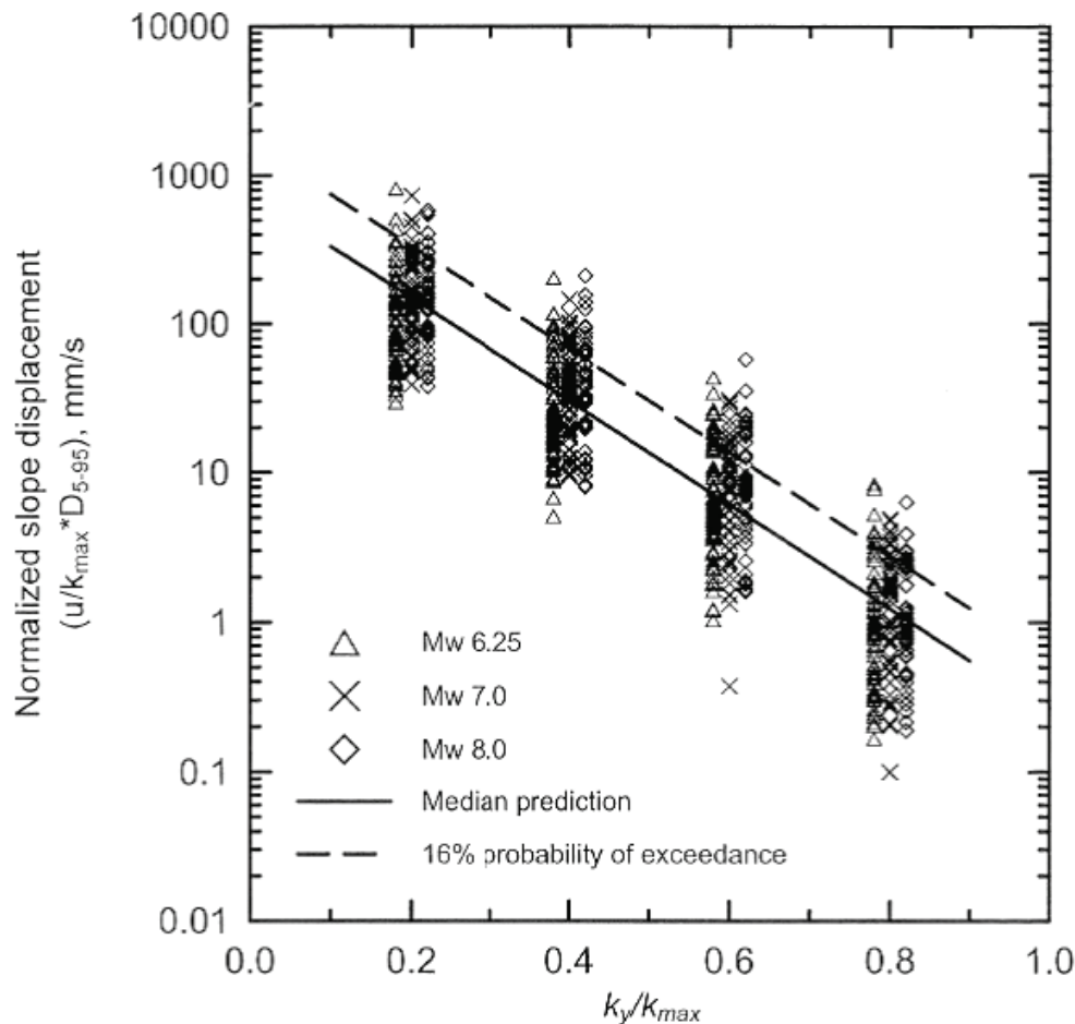
Figure 3 Normalized sliding displacement (Bray et al., 1998) as recommended by Blake et al. (2002).
