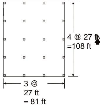
Figure 11 Plan view of reinforced concrete frame building.
