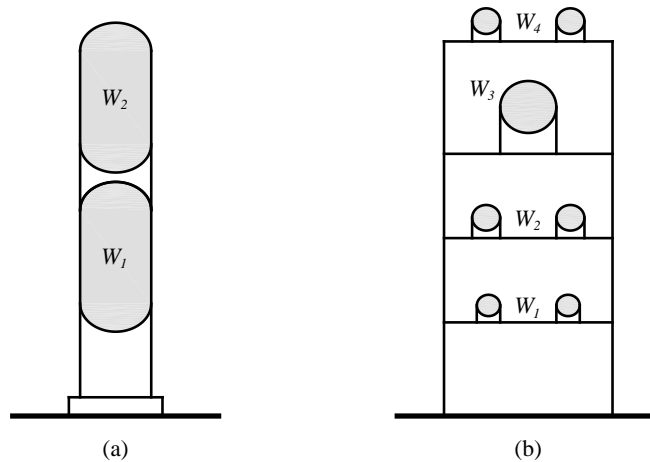
Figure C15.1-6 Mass irregularities.
