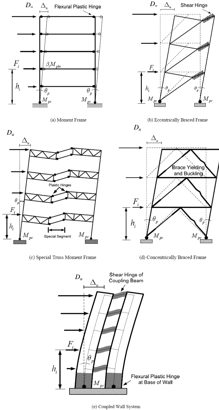
Figure 3 Desirable inelastic mechanisms.
