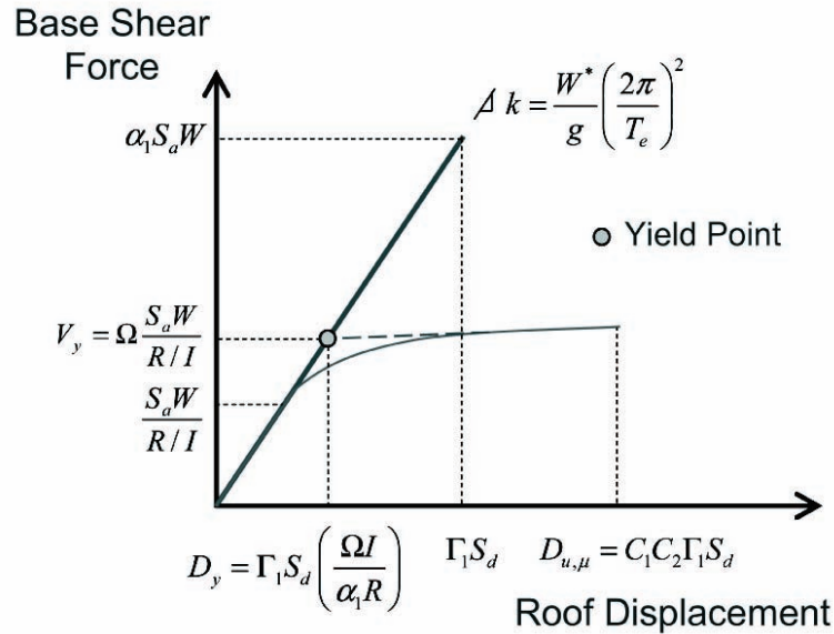
Figure 5 Response of elastic and yielding MDOF systems in the first mode. The “yield point” identifies the change in slope of a bilinear curve that is fitted to the capacity curve over the applicable range of displacement response. \Omega represents the actual overstrength factor, not the value \Omega_n provided in the 2003 NEHRP Recommended Seismic Provisions.
