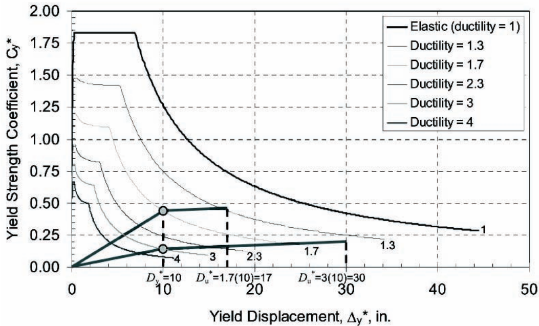
Figure 15 Yield point spectra.
