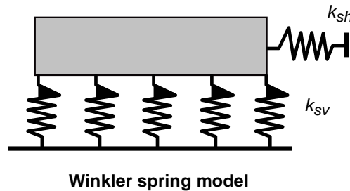
Figure C-A7.2.3-4.
