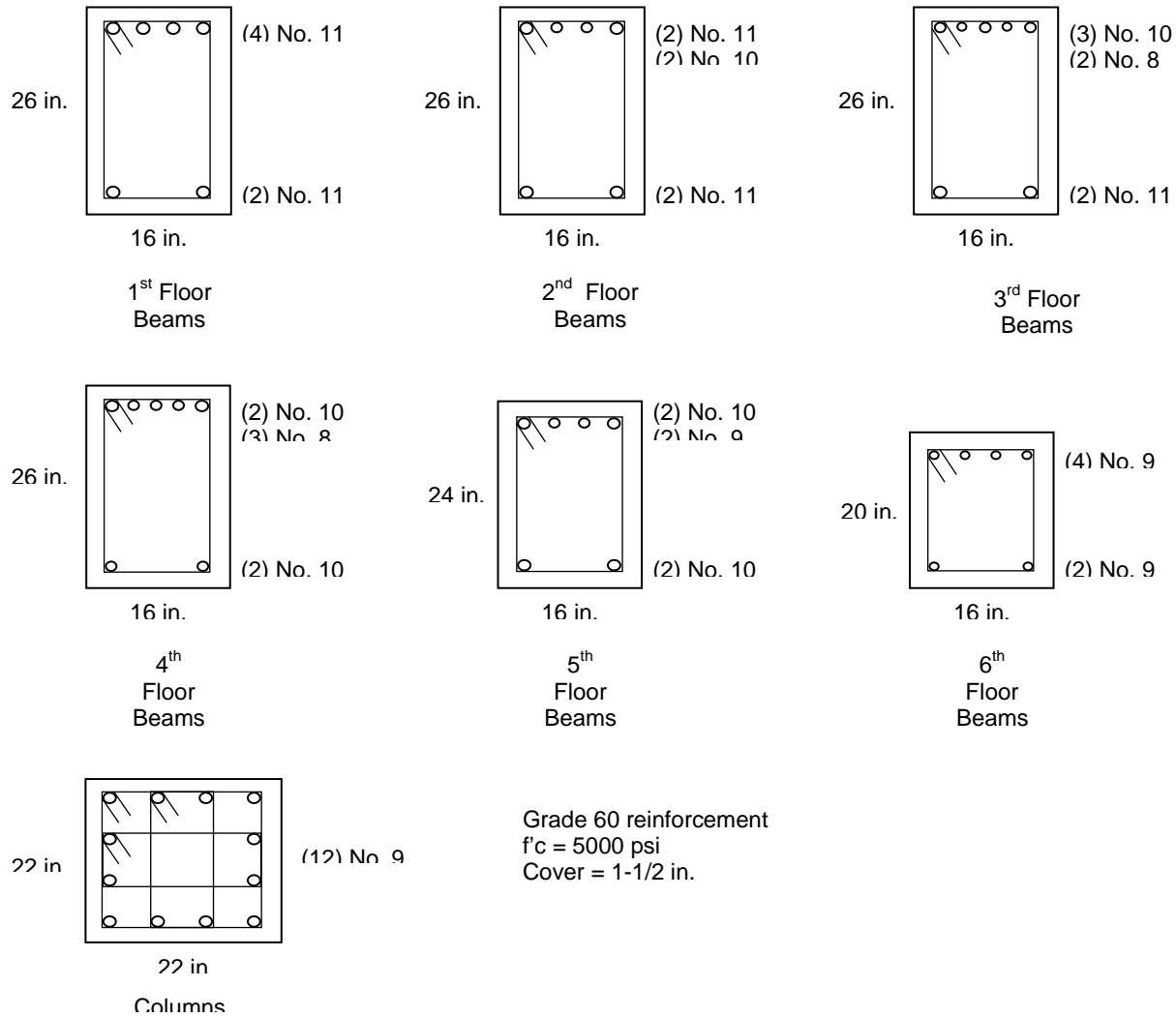
Figure 13 Beam and column section designed in the reinforced concrete frame example.
