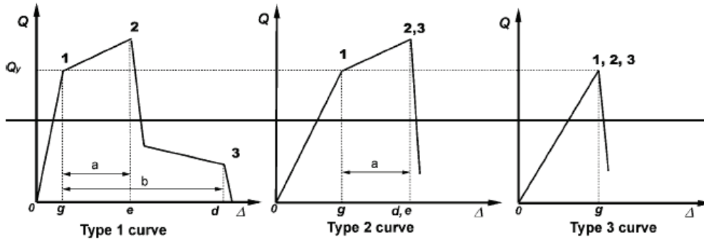
Figure A4-1 Connection classification per ASCE/SEI 41 procedures.
