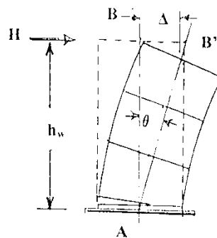
Figure C14.2.4.2.2-1 Definition of drift ratio \theta .
