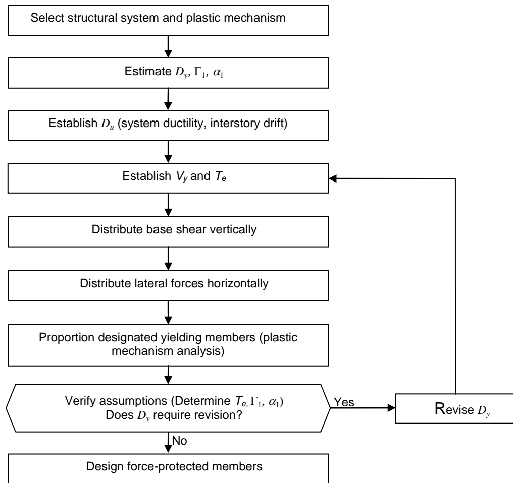
Figure 2 Steps in the design process.
