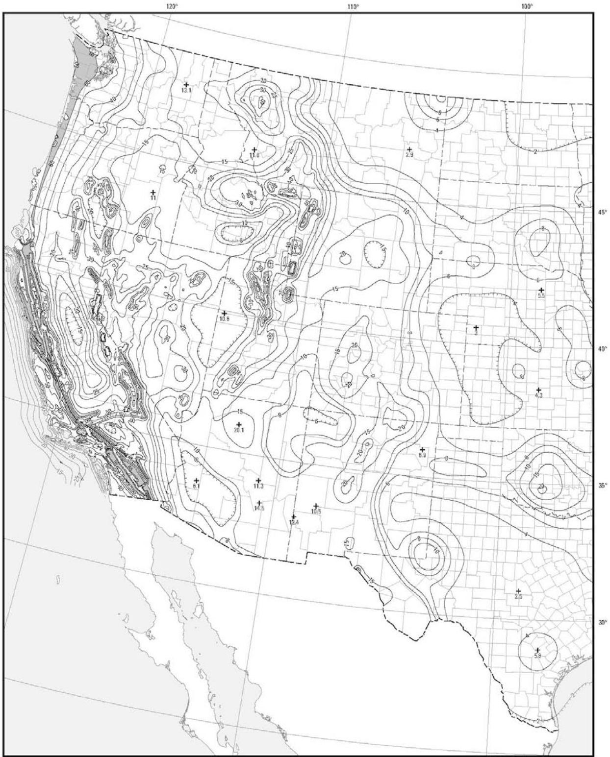
Figure 22-8 MCE geometric mean PGA, %g, Site Class B for the conterminous United States
