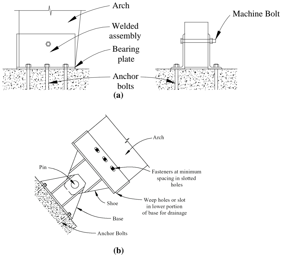
Figure C1.1.1 (a) Typical arch base with thru-bolt and (b) arch base with true hinge.
