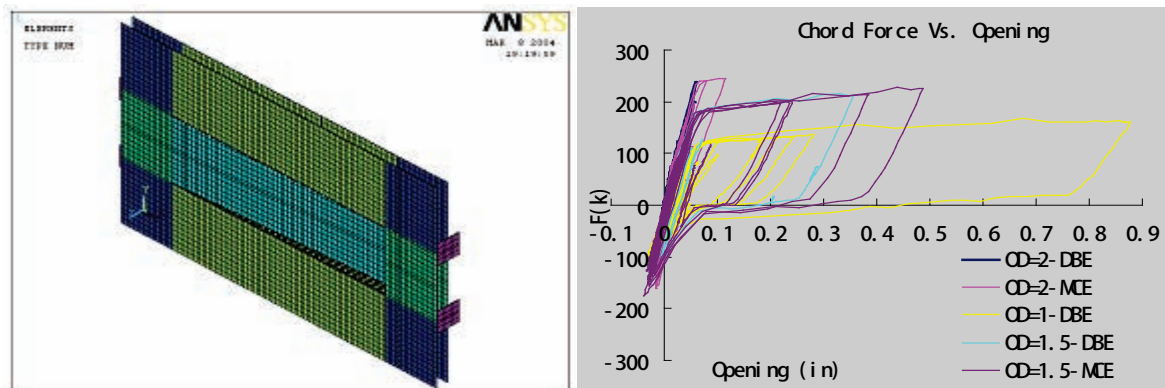
Figure A2-3 Schematic of 3D-FE model (left) and sample results for chord force vs. opening (right).
