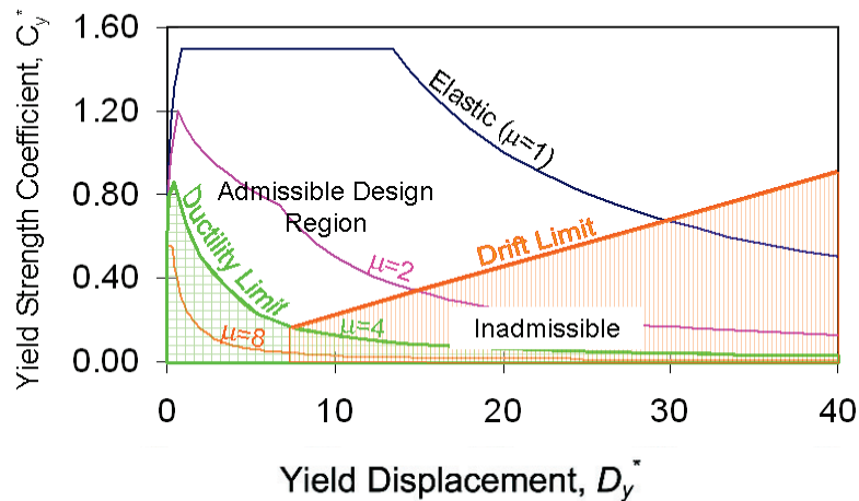
Figure 1 Limits on ductility and drift demands are used to establish admissible and inadmissible design regions. SDOF and ESDOF oscillators that have yield points located within the admissible design region satisfy the ductility and drift limits shown.
